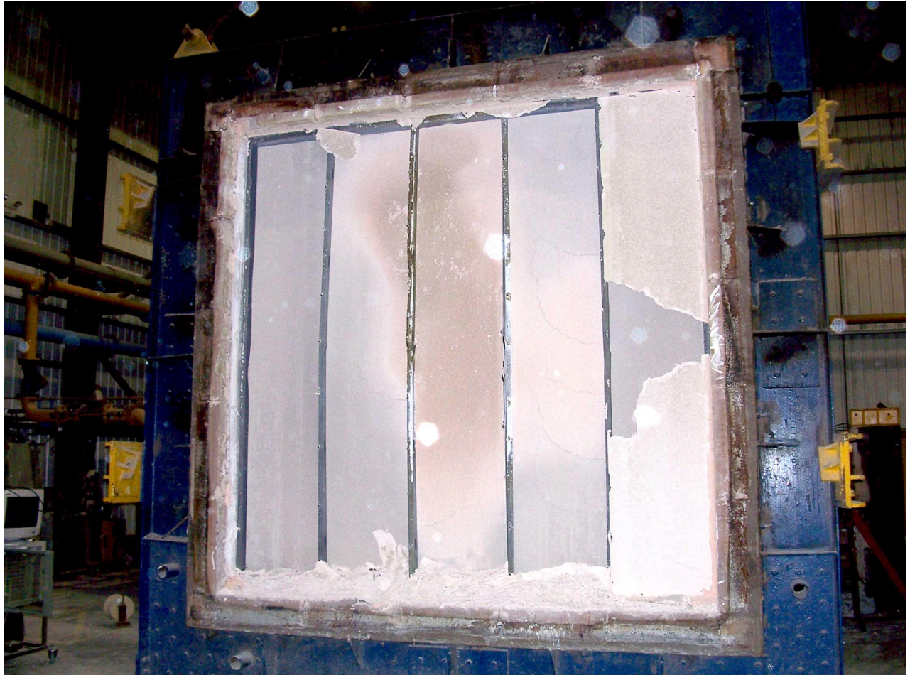
Photo 5 Exposed face of specimen after test.
