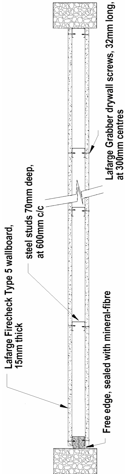
Figure 2 Section view through specimen.
